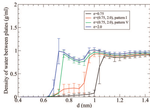
Figure 4. Density of water between two plates where particles are the same (black, blue) and where particles are distributed in pattern I (red) and in pattern V (green). Here the “hydrophilic sites” on the plates are neutral LJ particles with \varepsilon = 2.0 kJ/mol, and the “hydrophobic sites” are neutral LJ particles with \varepsilon = 0.75 kJ/mol.
