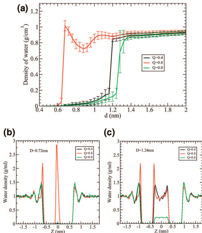
Figure 5. (a) Density of the water molecules confined between two plates which form a Janus interface, for different hydrophilicity (magnitude of the partial charge Q ) of the hydrophilic plate (plate1, see Figure 1b). Red corresponds to partial charge of Q = 0.8 e , black for Q = 0.4 e , and green for Q = 0.0 e in which case plate 1 is purely hydrophobic. (b) The density profile of the water molecules along z axis of the simulation box when the interplate distance d is 0.72 \text{ nm} . The origin z = 0 \text{ nm} is the middle point of two centers of mass of two plates, and the hydrophilic plate is located at the negative values of the z axis of the simulation box with |X| < 1.1 \text{ nm} and |Y| < 1.1 \text{ nm} (in the XY plane) are considered in these plots. (c) The same as (b) except for d = 1.24 \text{ nm} .
