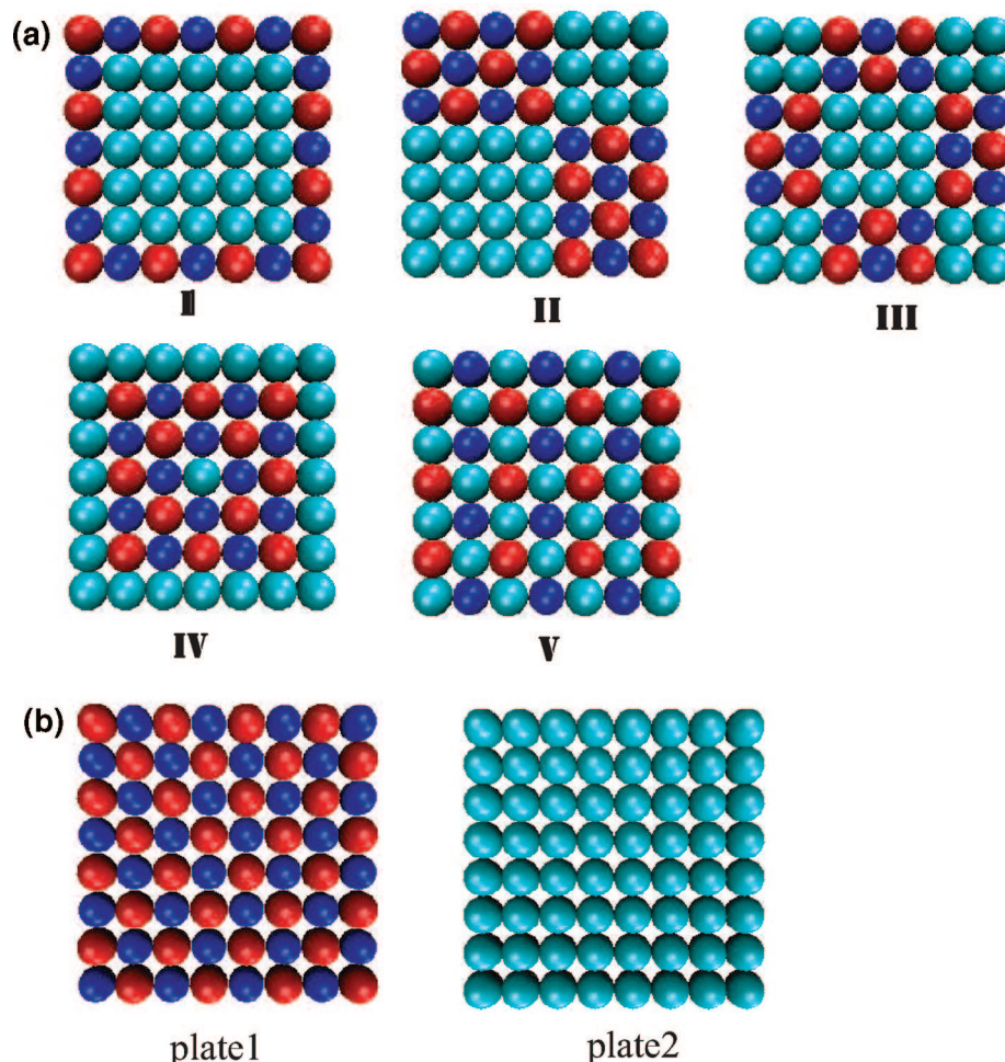
Figure 1. (a) Hybrid hydrophobic/hydrophilic plates with five different patterns of particle distribution, pattern I–V. (b) Janus faced plates: plate 1 and plate 2. The sphere in cyan represents hydrophobic particle, blue represent positive charged particle, red represent negative charged particle.
