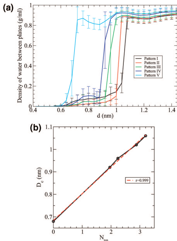
Figure 2. (a) Density of water in the interplate region for pattern I–V as a function of interplate distance when Q = 0.4 e for hydrophilic particles. (b) The critical distance of dewetting transition as a function of the average number of hydrophobic nearest neighbors for each pattern. The red line is a linear fitting to the curve with correlation coefficient r of 0.999.
