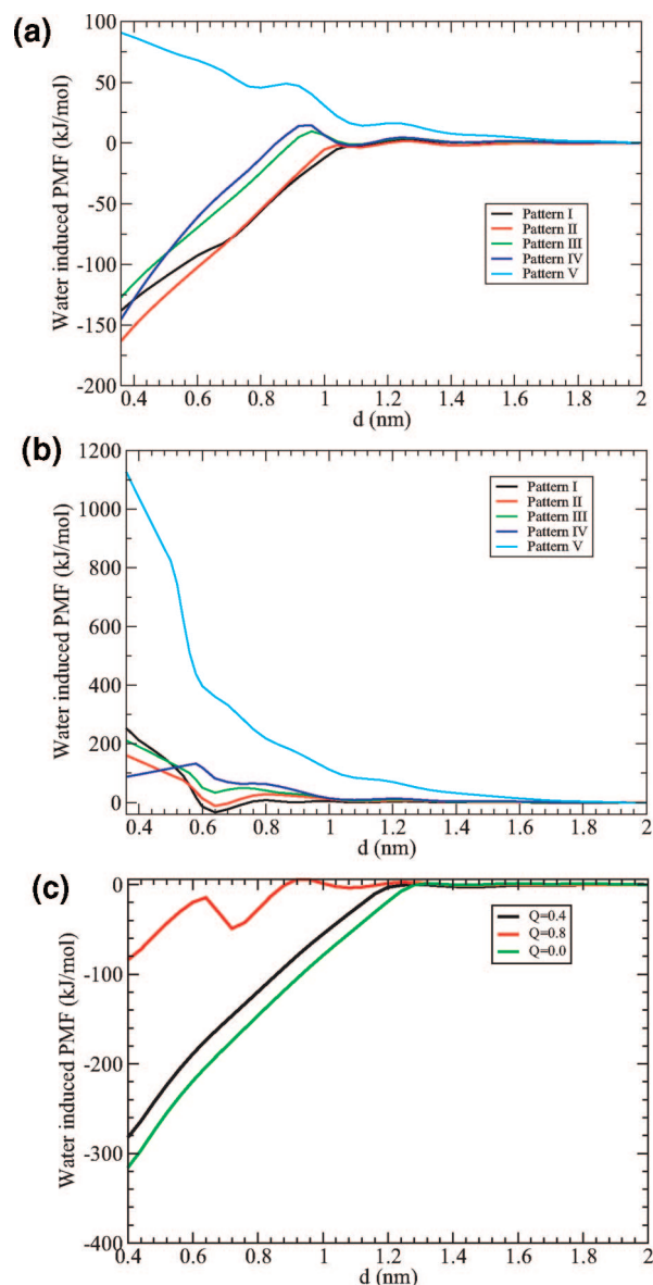
Figure 6. (a) Water induced PMF of two hybrid plates for pattern I–V as a function of interplate distance when Q = 0.4 e for hydrophilic particles. (b) The same as (a) except that the charge of hydrophilic particles is Q = 0.8 e (c) The water induced PMF of two plates which form Janus interfaces as a function of interplate distance with respect to different partial charge Q of the charged particles on plate 1 (see Figure 1b). Black is for partial charge Q = 0.4 e , red is for Q = 0.8 e , and green is for Q = 0.0 e in which case plate 1 is purely hydrophobic and identical to plate 2.
