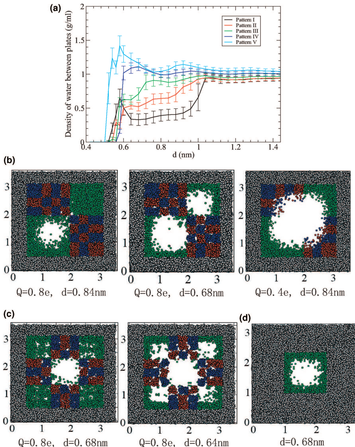
Figure 3. (a) Density of water in the interplate region for pattern I–V as a function of interplate distance when Q = 0.8 e for hydrophilic particles. (b) The view of a slab of water between two plates for pattern II. The water molecules are superimposed for 150 frames and are classified by different color based on their location. Water between opposite hydrophobic domains are represented in green; water between charged domains are in red and blue; water in the bulk are in silver. (c) the same as (b) except for pattern III. (d) the same as (b) except for the system of two plates, each of which is composed of 9 hydrophobic particles arranged in 3 \times 3 square lattice with a bond length of 0.32 nm.
