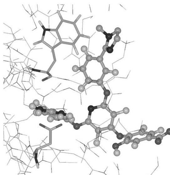
Figure 10. The binding site of trypsin bound to I1. The inhibitor and the residues Asp189 and Trp215, that form hydrogen bonds with the benzylamidine ring of I1, are emphasized.
